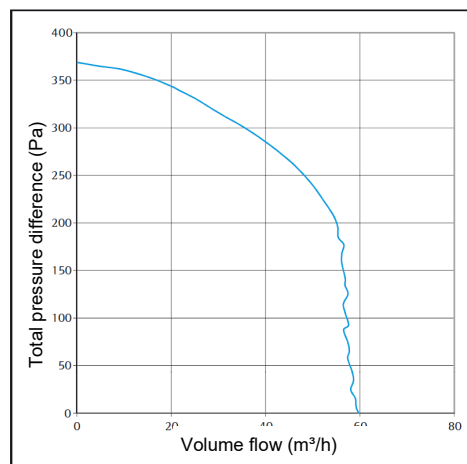
Pressure-volume-characteristic curve 3/UP-2BR
